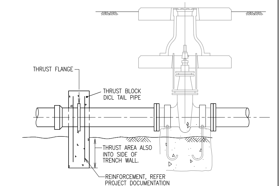
SLUICE VALVE (ø200 & GREATER - SOFT CLAY)
