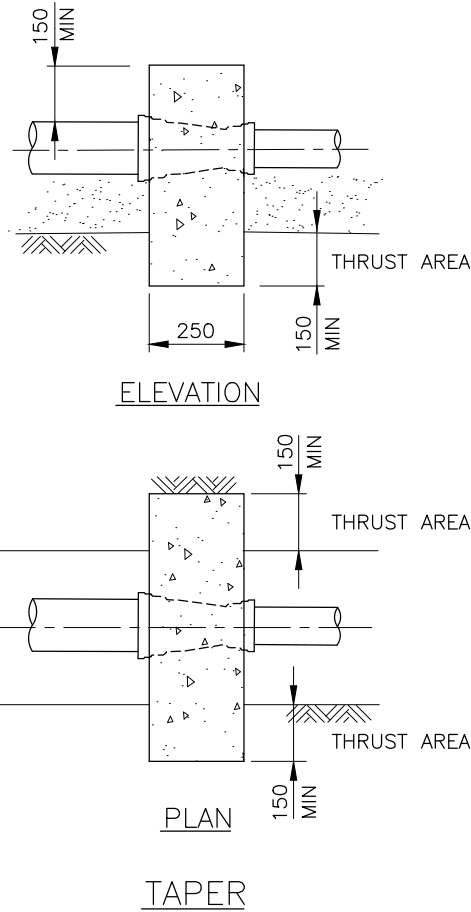
CONCRETE VOLUMES TO COUNTER THRUST (m 3 PER 1200kPa TEST PRESSURE)
