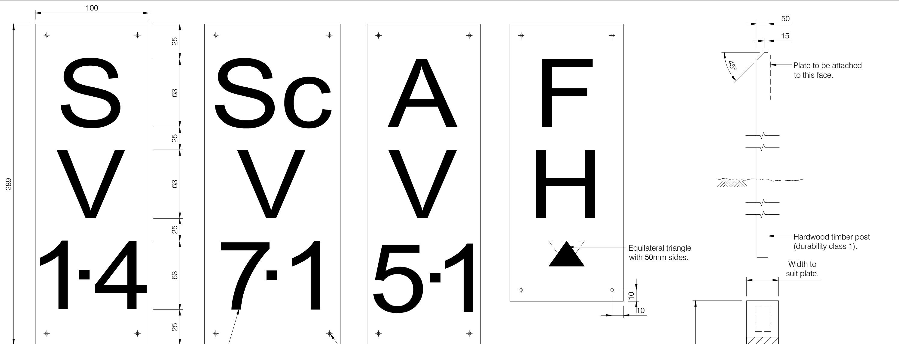
STOP VALVE
