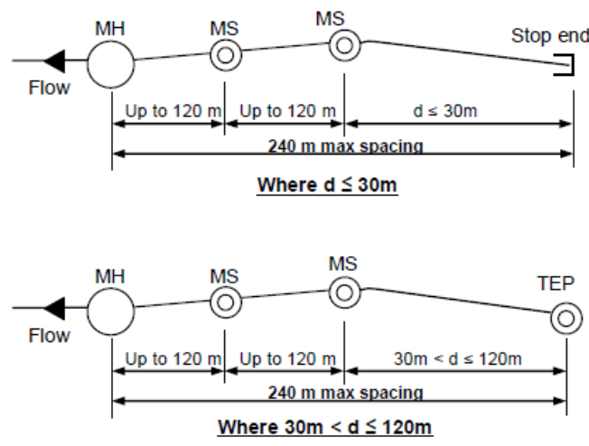
FIGURE 6.1 MULTIPLE MS BETWEEN MH AND “LAST” MH/MS/TEP (diagrammatic only)
