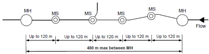
FIGURE 6.2 MULTIPLE MSs BETWEEN CONSECUTIVE MHs (diagrammatic only)
